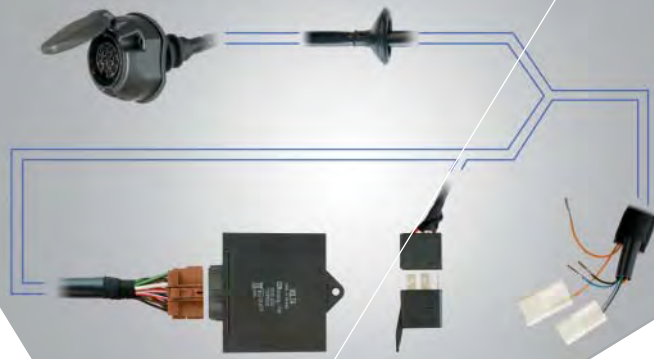
Tow bar wiring harness
