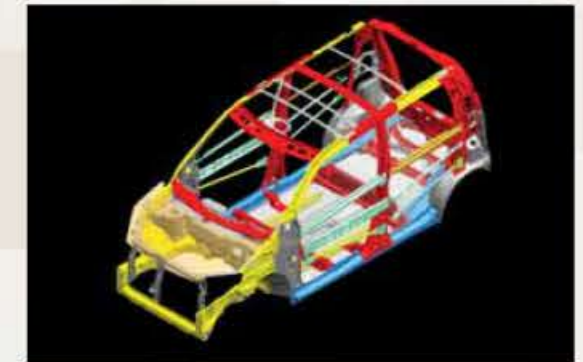
Energy absorbing body structure for safer drives
