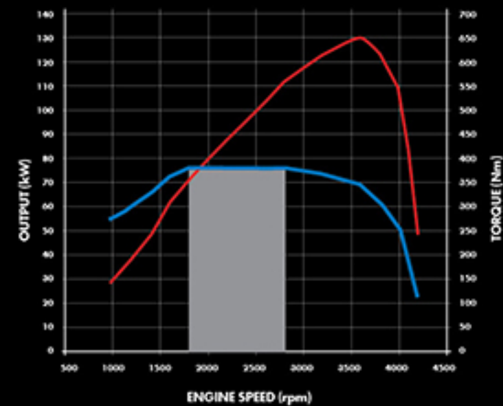
Flat Torque Curve
