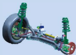
MCPHERSON STRUT IN THE FRONT
