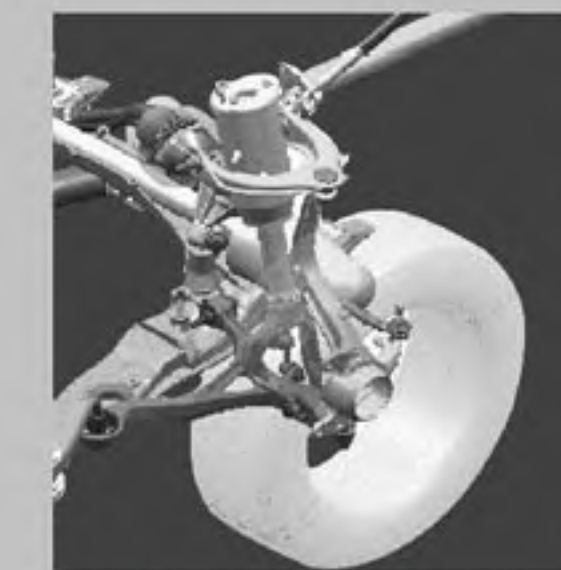
Double Wishbone Suspension
