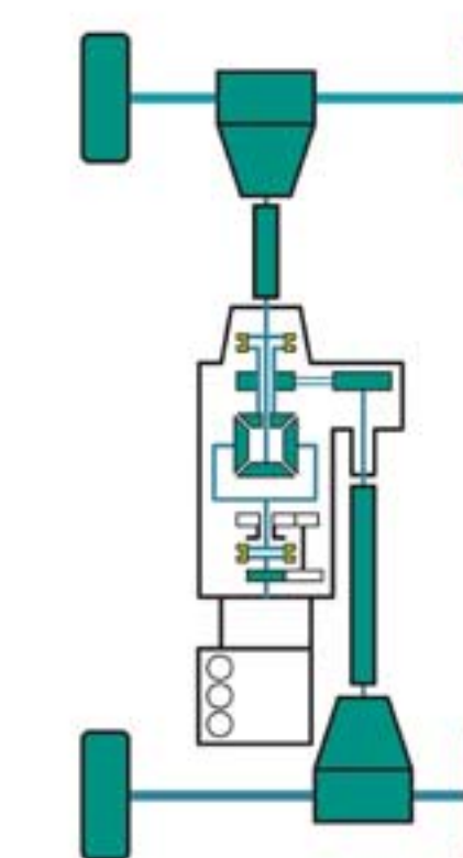
4 High Lock: Central differential locked. Power sent to front and rear wheels equally. Switch to this mode for medium off roading.
