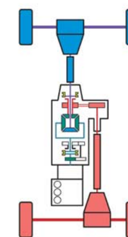
4 High: Central differential on. Power is sent to all wheels, all the time. Switch to this mode for normal driving.
