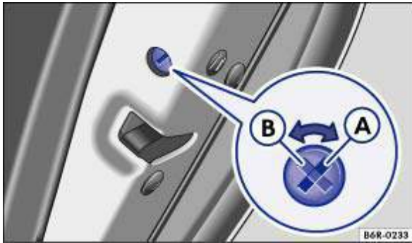
Fig. 32 In the right rear door: childproof lock (A) switched off, (B) switched on
