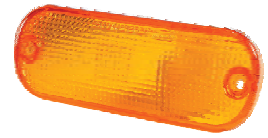
7055-615 Lens for Front Combination RH Type II 7056-615 Lens LH
