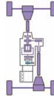
4 Low Lock: Central differential locked. Power sent to front and rear wheels equally but after increasing the torque using a 'traction enhancer'. Switch to this mode when stuck in mud, sand or snow.
